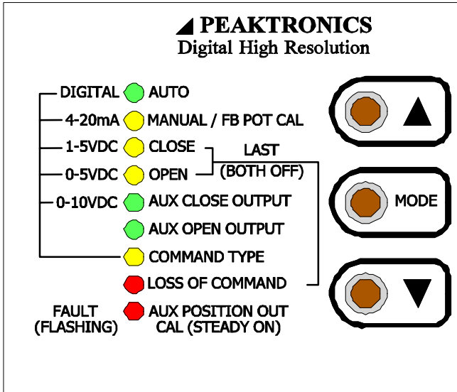
FRONT PANEL
