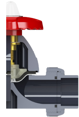
Weir Type Design Precise chemical flow control
